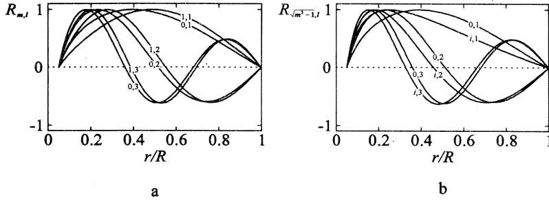
FIG. 4. Some of the radial parts of planar (a) and axial (b) modes, labeled by the indices k_m, l and k_{\sqrt{m^2-1}}, l for a capillary with planar radial structure and r_0 = 0.05R . In both cases the y axis units are arbitrary.
