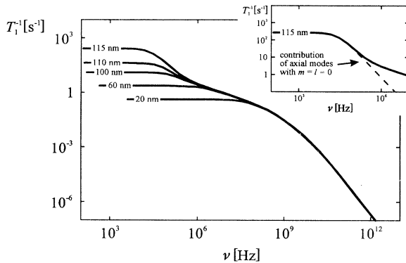
FIG. 6. Frequency dependence of the relaxation rate T_1^{-1} in capillaries with R=20, 60, 100, 110 , and 115 nm, parallel to the magnetic field. The parameters used in the calculation are T=293 K, S=0.4 , K=10^{-11} N, \eta=0.01 N s m ^{-2} , b=0.2 nm, r_0=5 nm; the length of the molecules is taken to be 2 nm. At larger radii, the low-frequency behavior is almost entirely due to the slowest axial modes, corresponding to m=l=0 (inset).
