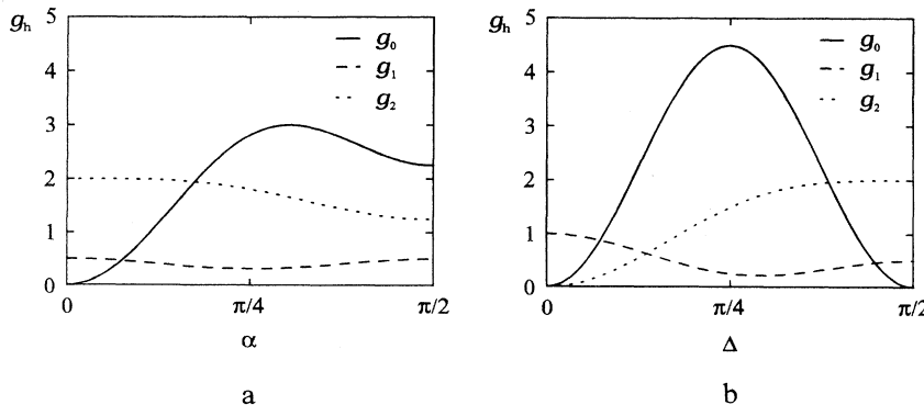
FIG. 5. Angular dependence of the spectral densities in planar radial structure (a) and uniform nematic structure (b). The functions g_h depend on the angle between the axis of the capillary and the magnetic field and the angle between the uniform director and the magnetic field, respectively. Note that g_1(\alpha) and g_2(\alpha) are more moderate than their uniform counterparts g_1(\Delta) and g_2(\Delta) .
